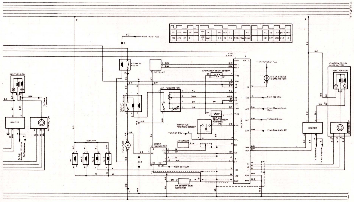
2 Typical early model (3S-FE and 3S-GE) starting and TCCS wiring diagram
